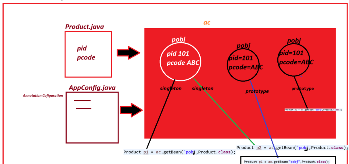
bean-scope-annotation-s16
